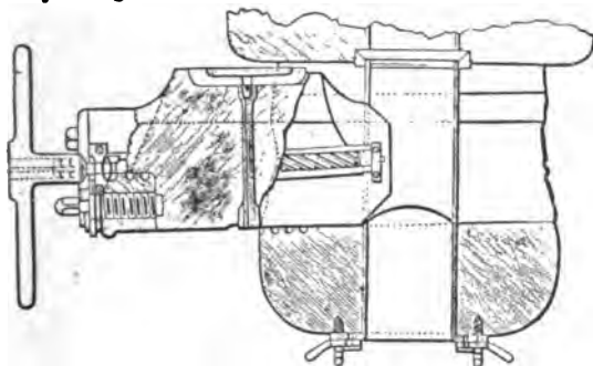
FIG. 44.—Krupp's breech action, cylindro-prismatic wedge.
