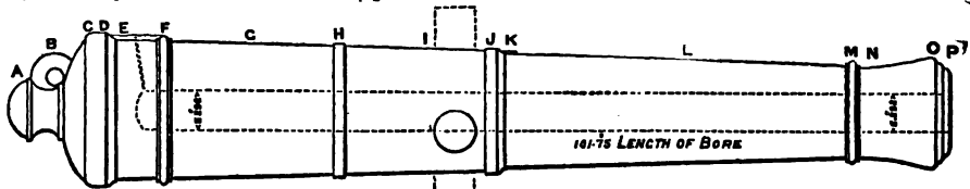
FIG. 19.—18-pounder Gun. A, button (cascable); B, breeching loop (do.); C, breech; D, base ring and ogee; E, vent-field; F, vent-field astragal and fillets; G, 1st reinforce; H, 1st reinforce ring; I, 2d reinforce; J, 2d reinforce ring and ogee; K, patch for foresight; L, chase; M, muzzle astragal and fillets; N, neck; O, swell of muzzle; P, muzzle mouldings.
