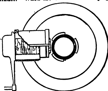
FIG. 46.—French breech action, interrupted screw.
