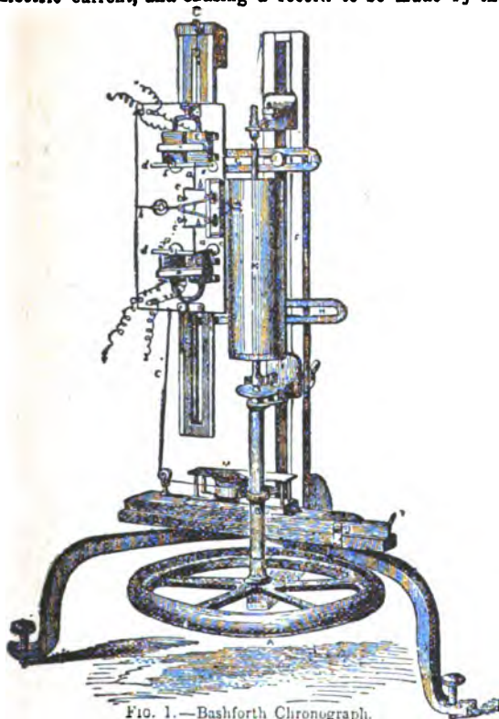
FIG. 1. — Bashforth Chronograph.
