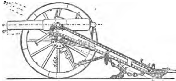
FIG. 38.—9-pounder Field Gun Carriage (elevation).
