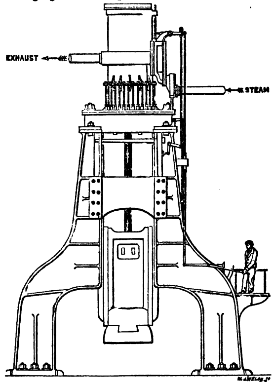
FIG. 4.—Steam Hammer.
