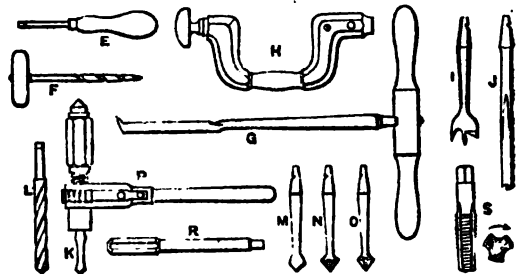
FIG. 5.—Boring tools.
