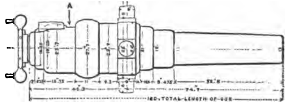
FIG. 41.—7-inch Armstrong Breech-loader.
