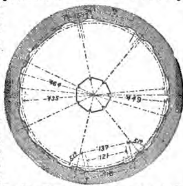
FIG. 17.—Henry rifling (true size and magnified).
