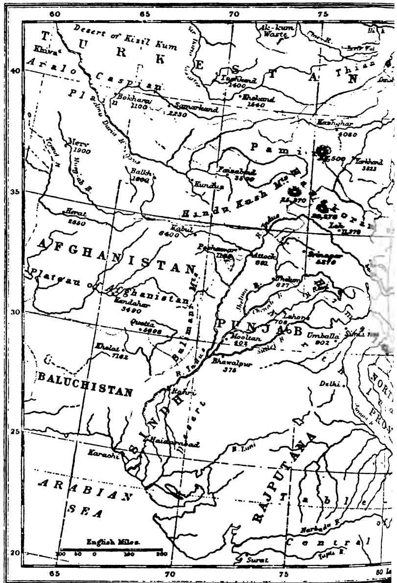
Sketch Map showing the connection between the Himalaya Mountains and the Arabian Sea. The darkest shade indicates the area the monsoon winds of which winds 10,000 feet, the
