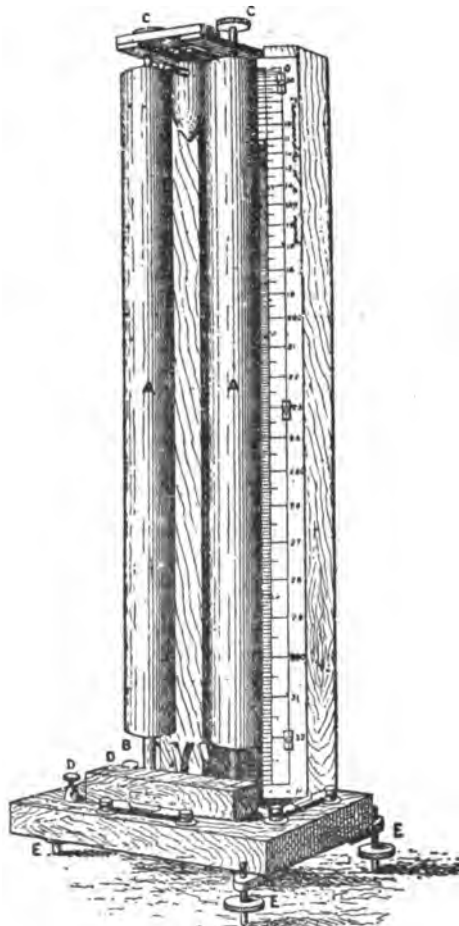
FIG. 12.—Watkin Chronograph.
