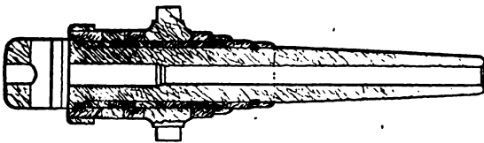
FIG. 40.—Section of Krupp Gun.
