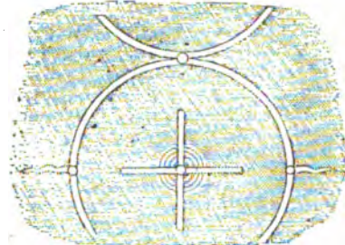
FIG. 4.—A system of lunar halos and paraselenæ figured in Buchan's Meteorology , p. 193.
