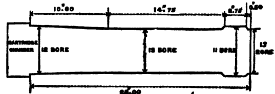
FIG. 9.—Double choke.
