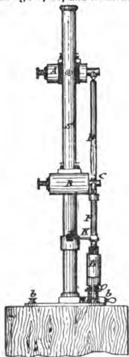
(Fig. 9.—Le Boulengé Chronograph, side view.
