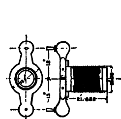
FIG. 42.—Breech Screw.
