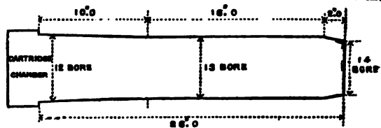
FIG. 8.—Plain choke.
