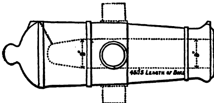
FIG. 20.—8-inch Howitzer.
