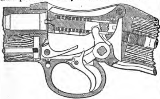
FIG. 14.—Martini breech action (closed).
