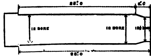
FIG. 10.—Greener's choke.
