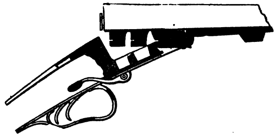
FIG. 11.—Treble grip snap action.
