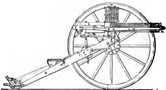
FIG. 20.—Gatling Gun.
