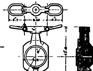
FIG. 43.—Vent Piece.
