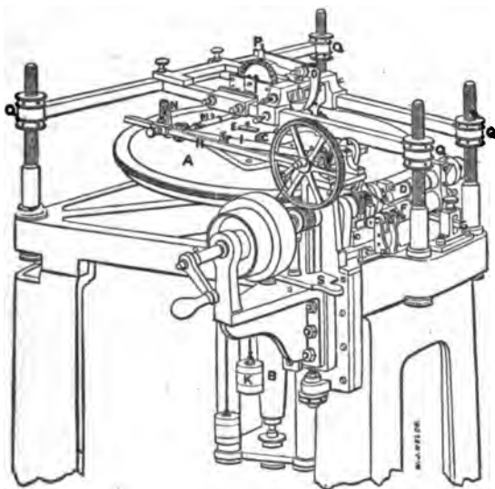
Dividing Engine.
