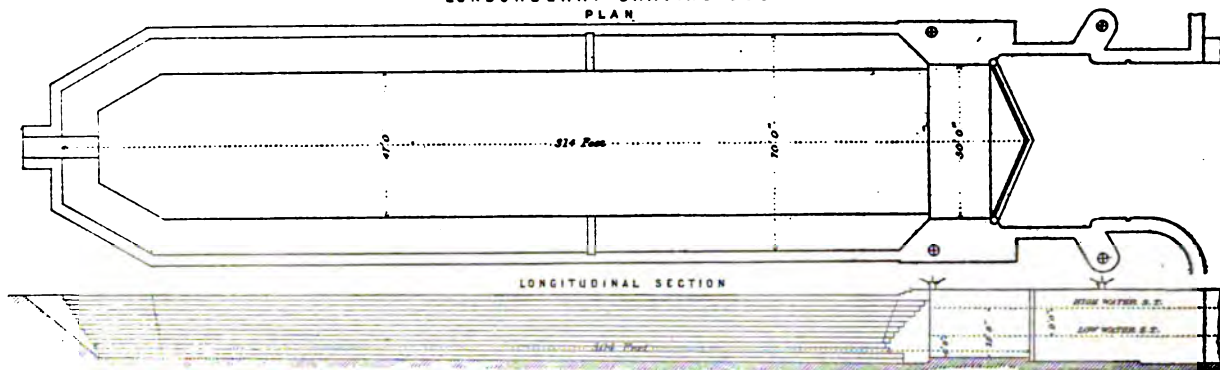
LONDON DERRY GRAVING DOCK PLAN
