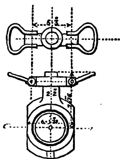
FIG. 27.—40-pounder Vent Piece.
