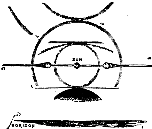
FIG. 1.—Solar halos and parhelia seen at Brighton, June 5, 1875, by F. E. Sawyer, from 4 to 5.45 p.m. The halo \alpha was a large one, having the zenith for its centre and going entirely round the heavens. It was a white band, and passed through the sun and the mock suns. The parhelia were of prismatic colours and had flaming tails.
