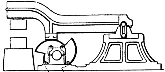
FIG. 2.—Lift Hammer.
