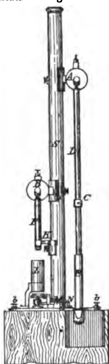
FIG. 10.—Le Boulengé Chronograph, front view.
